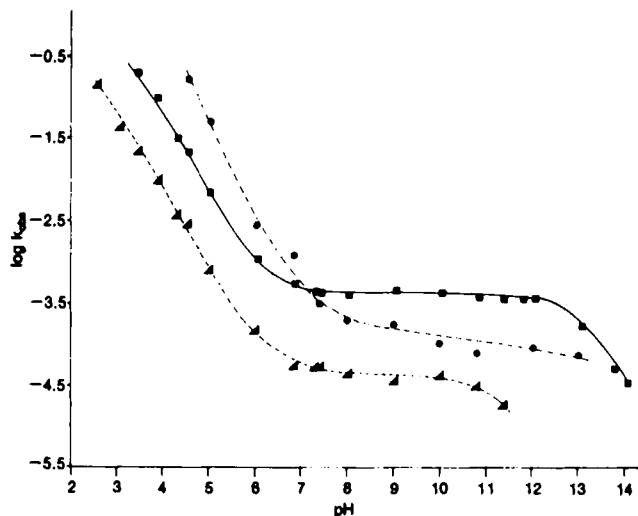
Figure 1 —Log k_{obs} -pH profile of I. Key: (■) in buffered aqueous solution at 25°C and \mu = 0.01 , calculated according to Eq. 1; (▲) in presence of 2 \times 10^{-2} M hexadecyltrimethylammonium bromide; (●) in presence of 2 \times 10^{-2} M sodium lauryl sulfate.
